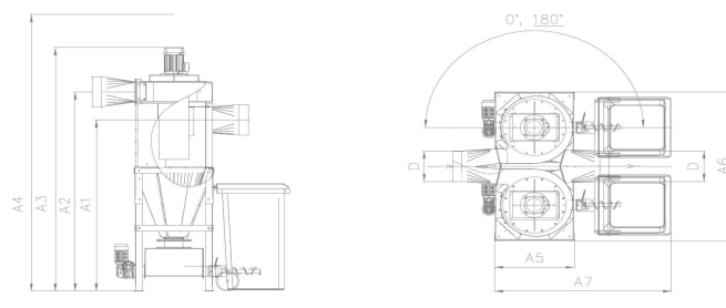
BF600-800-1000
