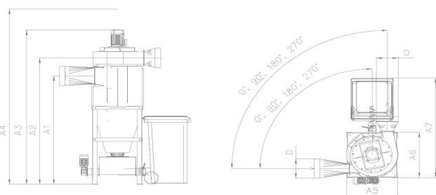
BF500
